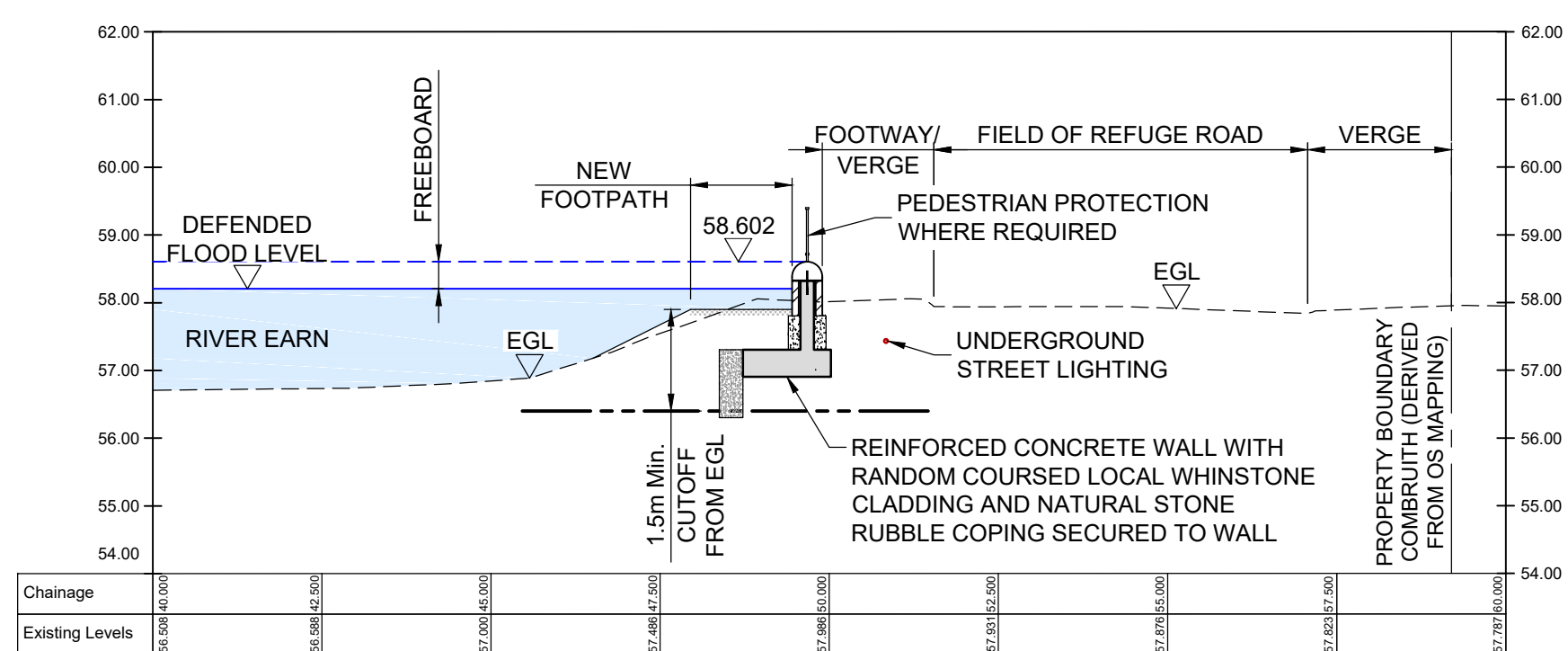
SECTION D-D SCALE 1:100
