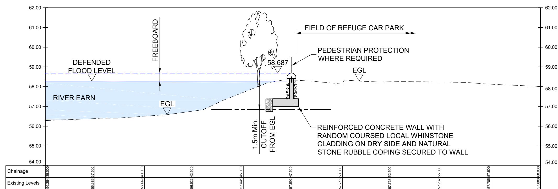
SECTION C-C SCALE 1:100
