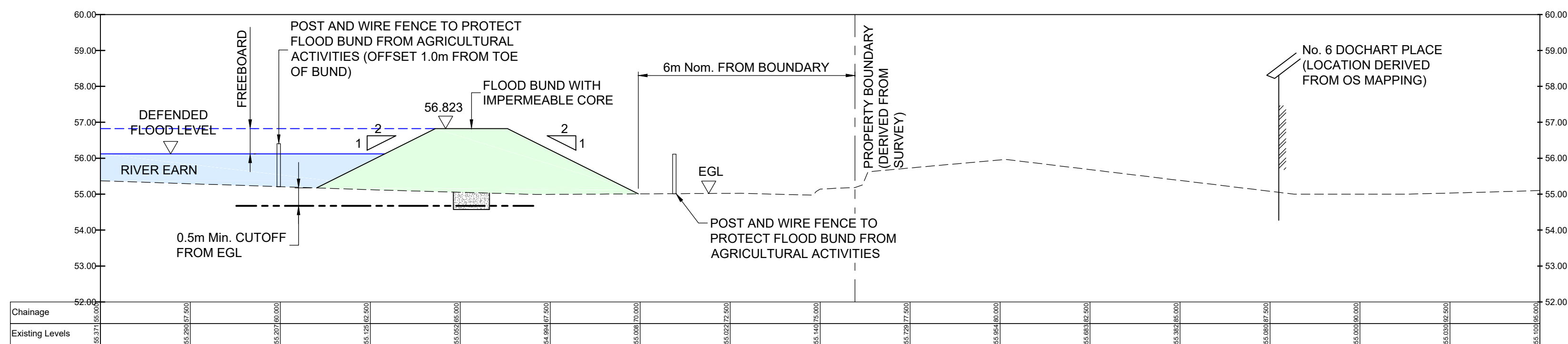
SECTION C-C SCALE 1:100
