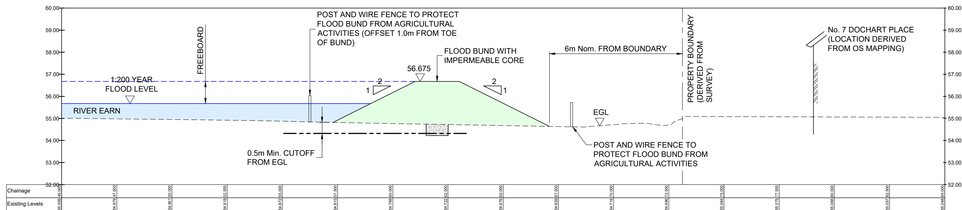
SECTION D-D SCALE 1:100
