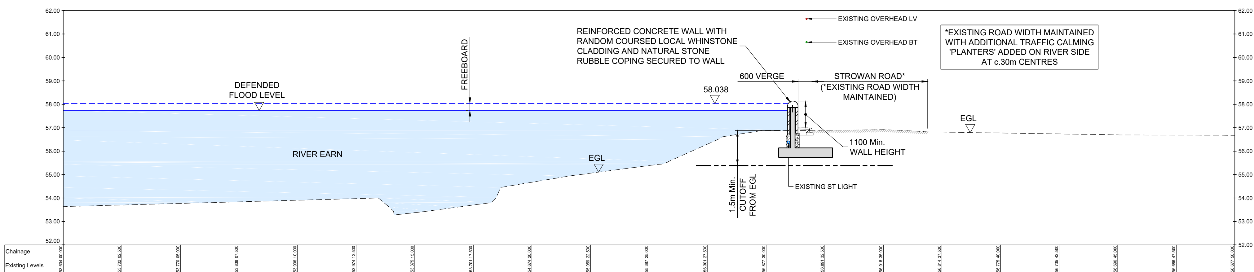
SECTION D-D SCALE 1:100
