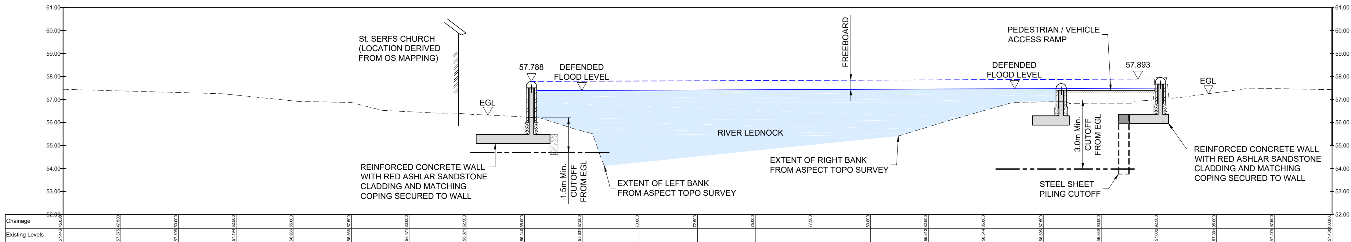
SECTION C-C SCALE 1:100
